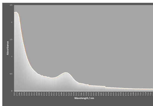
Figure 7. Rubus adenotrichus aqueous extract 4% w/w Uv-visible Absorption Spectrum.
