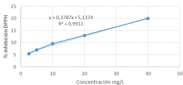
Figure 5. Percent Inhibition Curve by DPPH Quantification in Rubus Adenotrichus Aqueous Extract.
