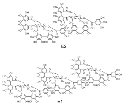
Figure 2. Ellagitannins detected in Rubus adenotrichus , (E1) Lambertianin C, \gamma (E2) Sanguin H-6. 7
